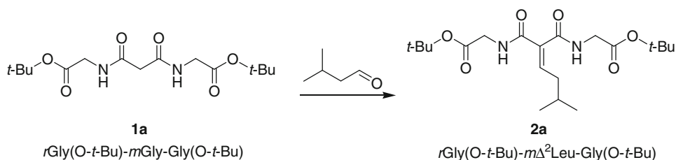
Scheme 3 Knoevenagel reaction on symmetric malonyl peptides
