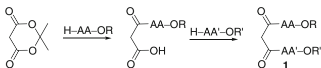
Scheme 1 Synthesis of malonyl peptides
