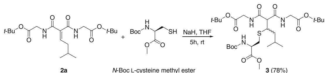
Scheme 5 Michael addition of a L-cysteine derivative
