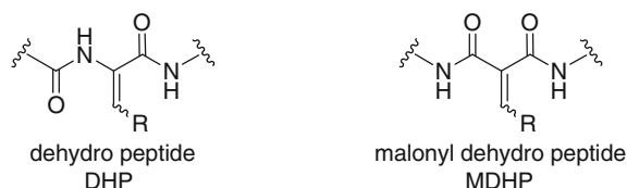
Fig. 1 Natural and malonyl dehydro peptides
