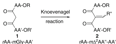
Scheme 2 Synthesis of malonyl dehydro peptides
