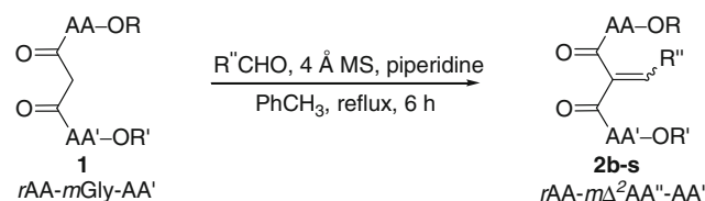
Scheme 4 Standard Knoevenagel condensation
